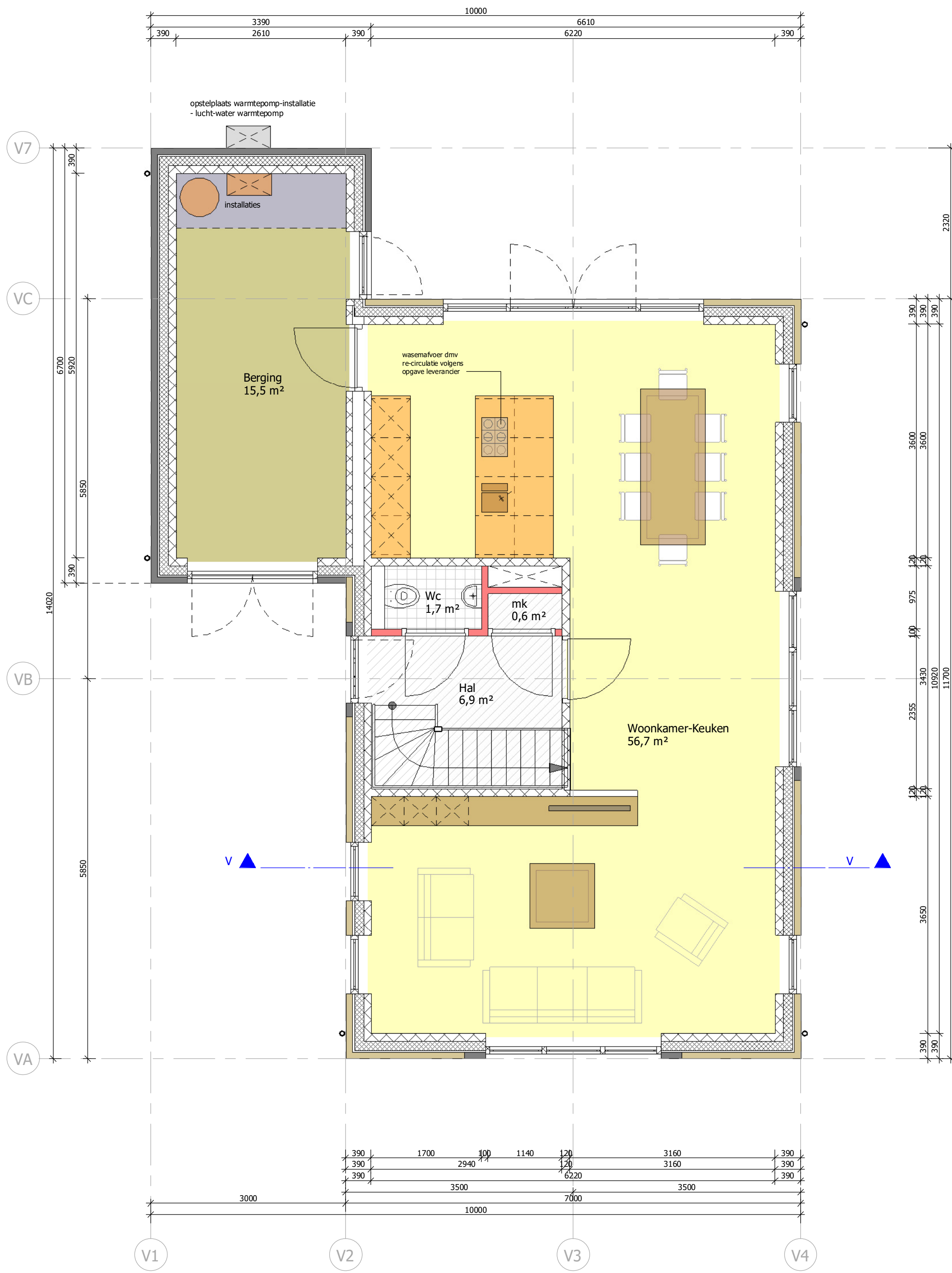
begane grond (1:50)
